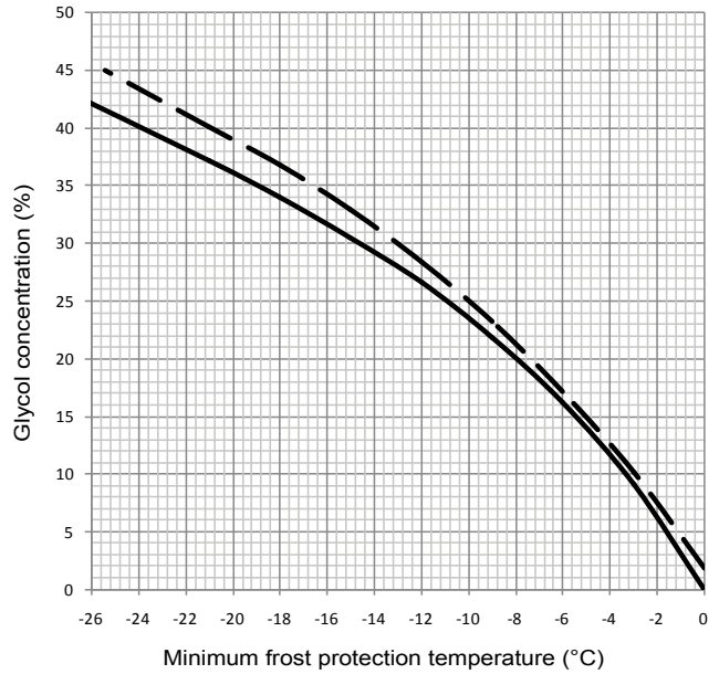
Freezing curve for Ethylene and Propylene glycol
