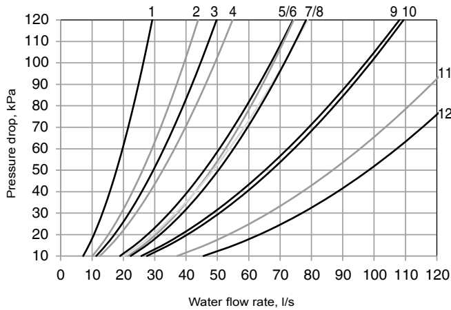
Units with two condenser passes (standard): 30XW--/30XWH-/30XW-P/30XWHP
