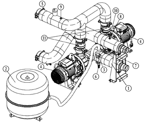
Hydraulic module - sizes 090-160 Dual pump and expansion vessel
