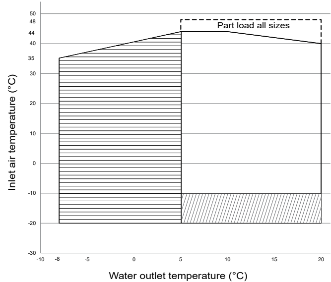
Operating map - unit 30RB option 16 30RB 040R-160R
