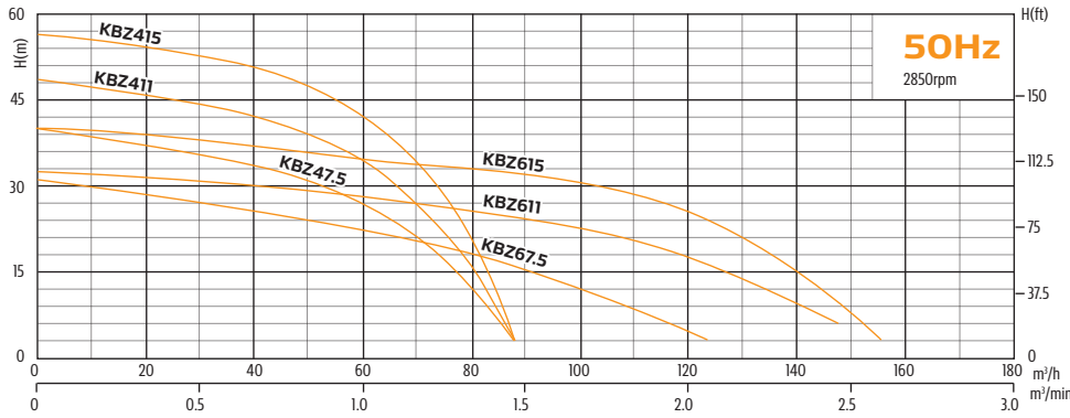
PERFORMANCE and SIZE CHART
