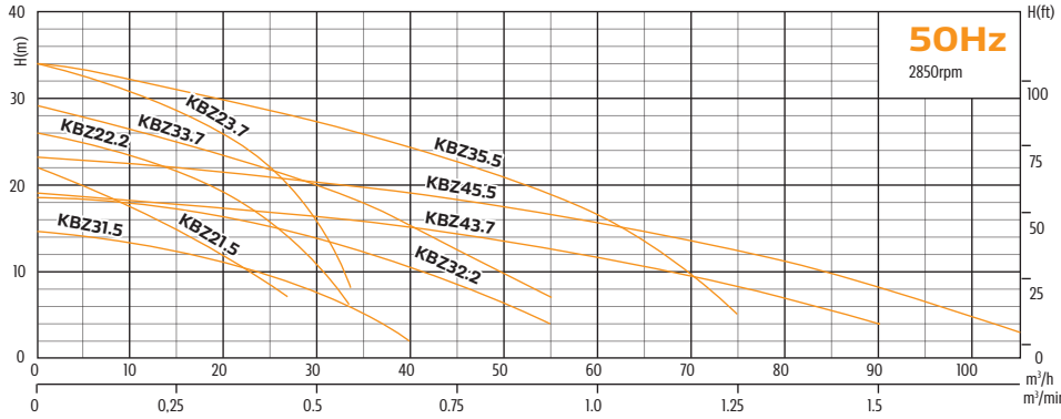
PUMP FLOW (Q) - PRESSURE (H) TABLE
